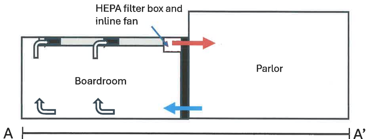
Figure 6. Ventilation schematic showing air quality control flow dynamics. Red arrows show upper filtration out of each room while blue arrows show fresh air intake. All rooms filter back into the parlor's main filtration system.
